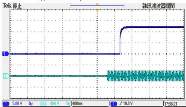
Figure 7 : CH1 = Vout, CH3 = 115V Input
