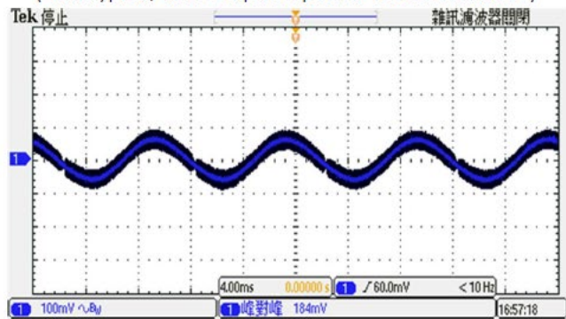
Figure 8 : Output Voltage Ripple & Noise at full load.
